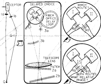
Delayed-Choice Experiment von J. A. Wheeler.
