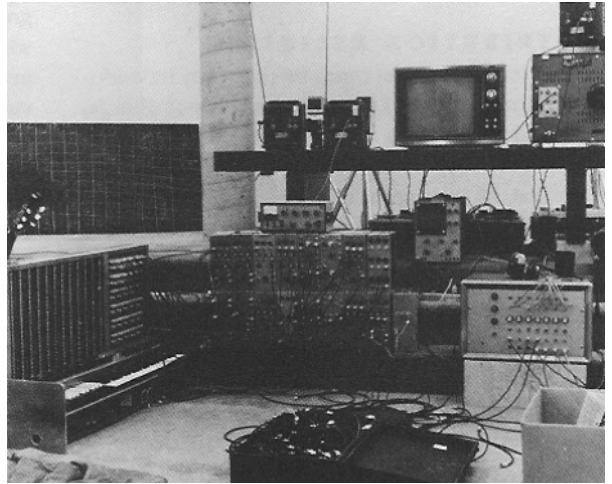
Left: Dan Sandin with the IP (Image Processor, 1972, Chicago). Below: Dan Sandin's IP in studio with other instruments.
